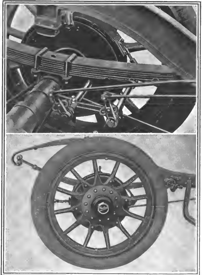
Fig. 11—Brake adjustment details on the different Overland models for 1912 Fig. 12—Heavier wheels are used on the 1912 Overland models on all chassis
